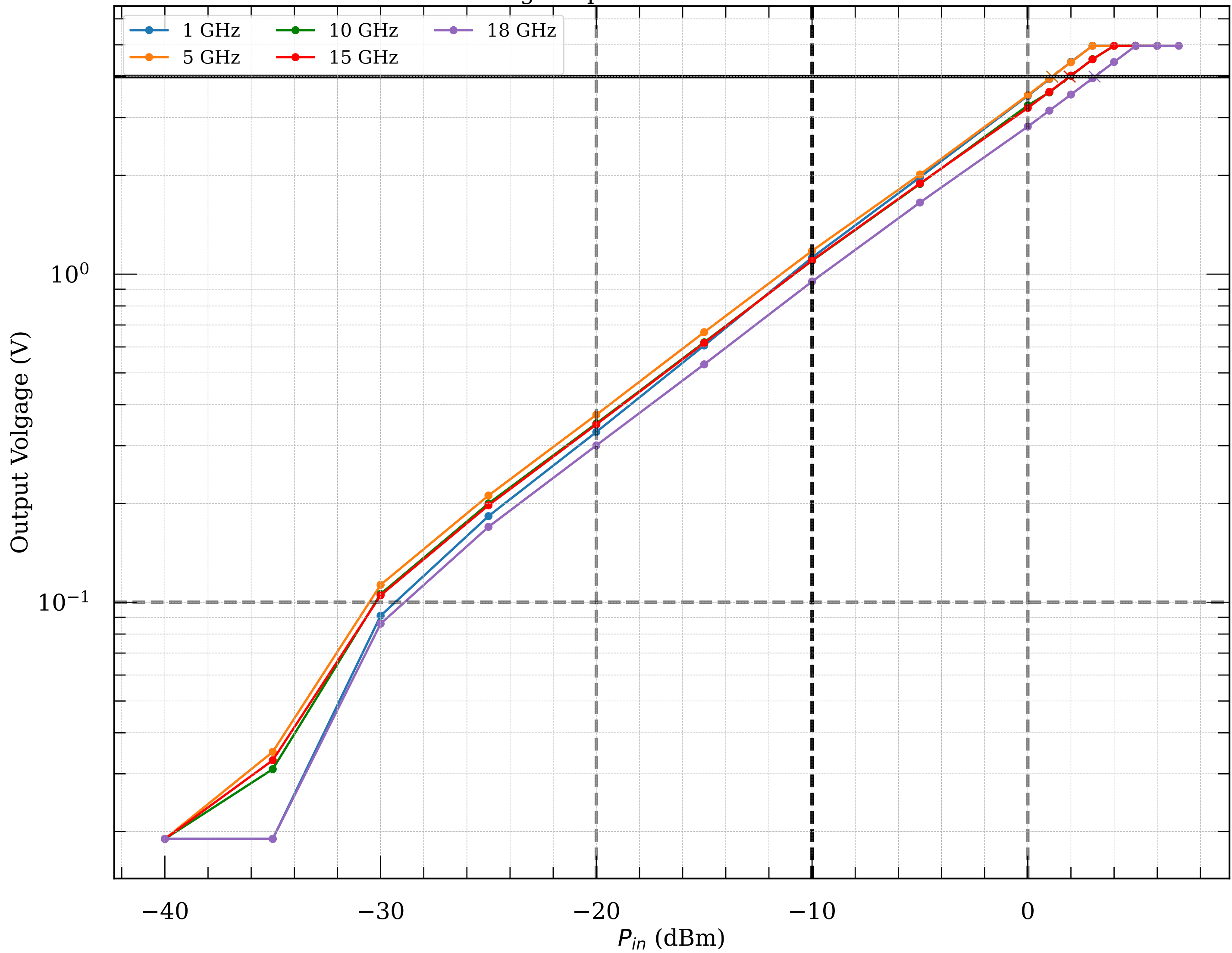
Measured voltage-to-power curve of detector module070
